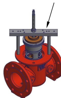
Disassembling tool F0001238 (not supplied with the pressure reducing valve 576)
